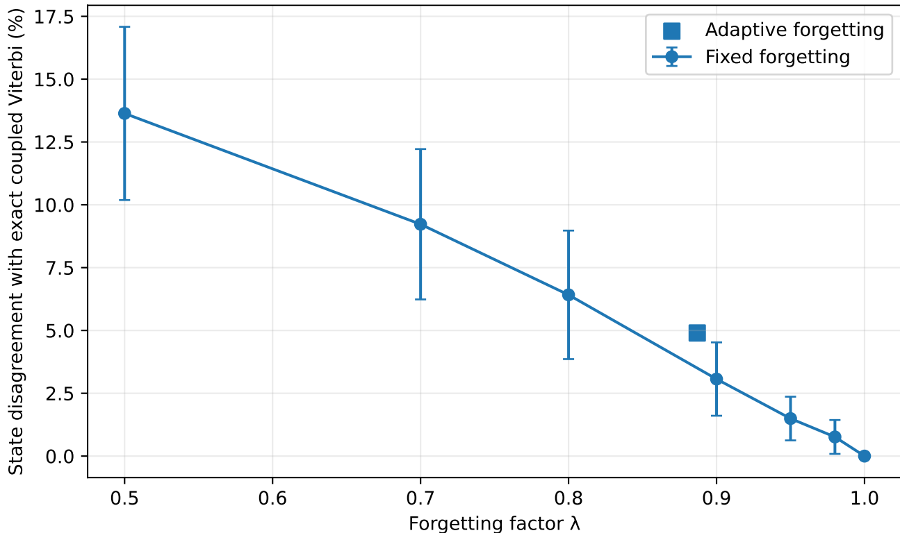
Approximation cost of forgetting on an exactly solvable coupled system
