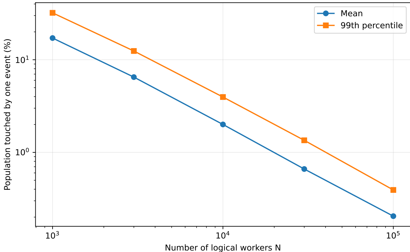
Adaptive forgetting: affected population fraction vanishes with N
