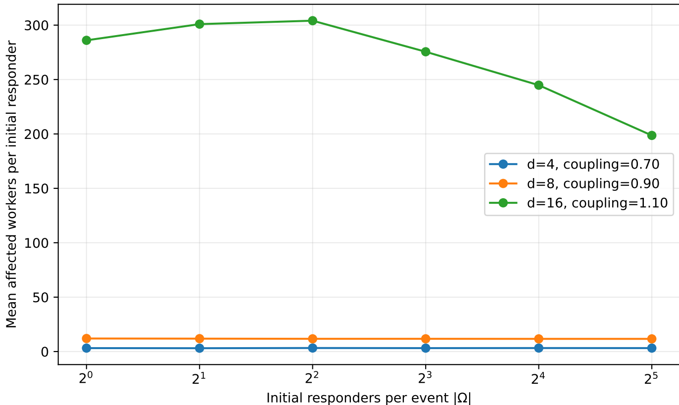
Cascade amplification remains the relevant quantity
