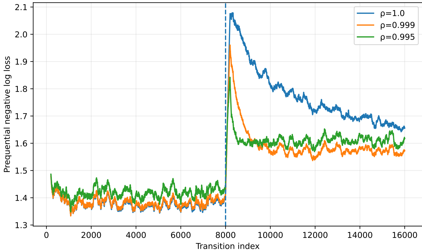
Online transition learning under abrupt drift
