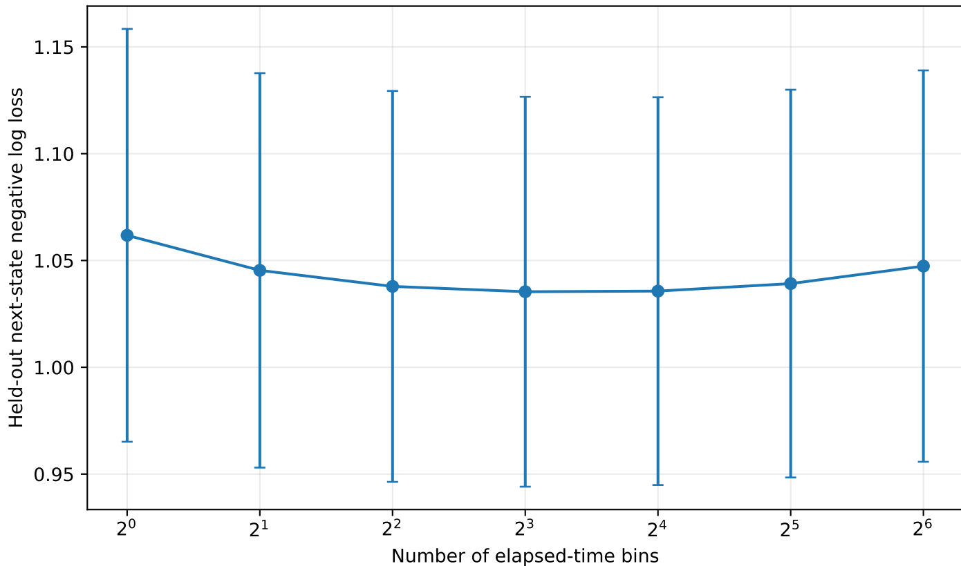
Predictive price of coarse elapsed-time binning
