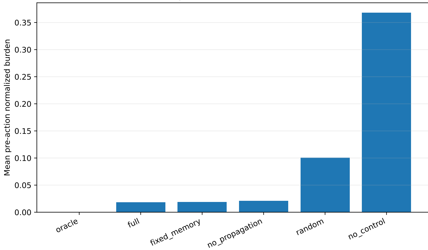
Integrated architecture ablation
