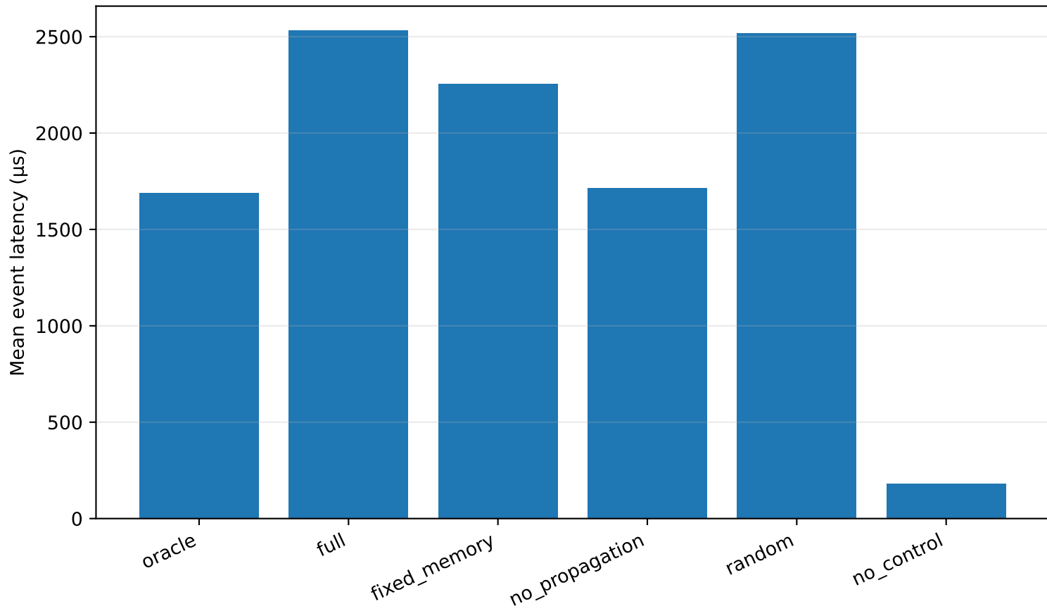
Integrated controller overhead
