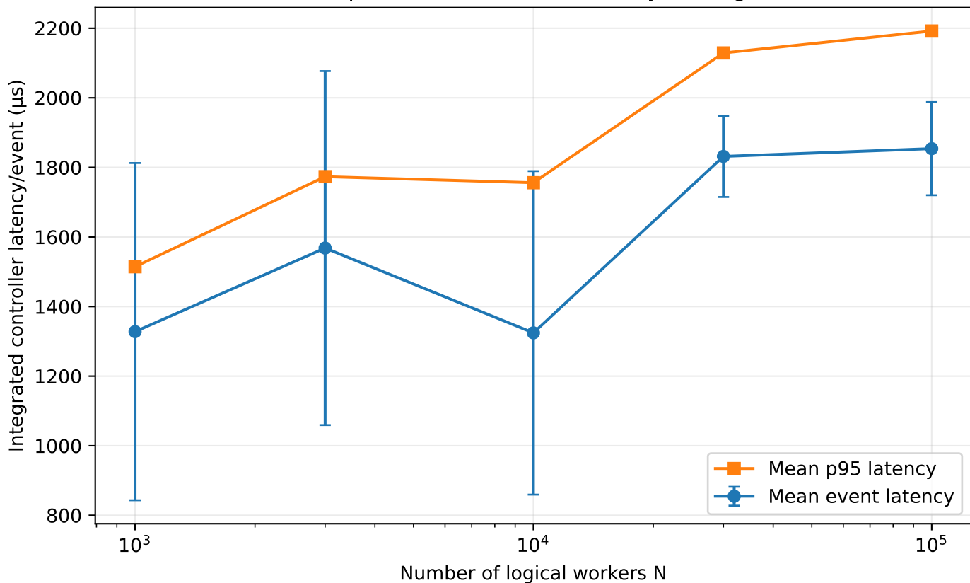
Replicated end-to-end latency scaling
