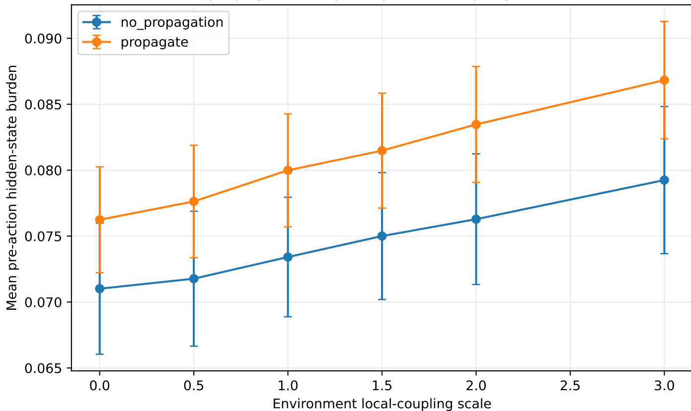
State propagation helps only when coupling warrants it
