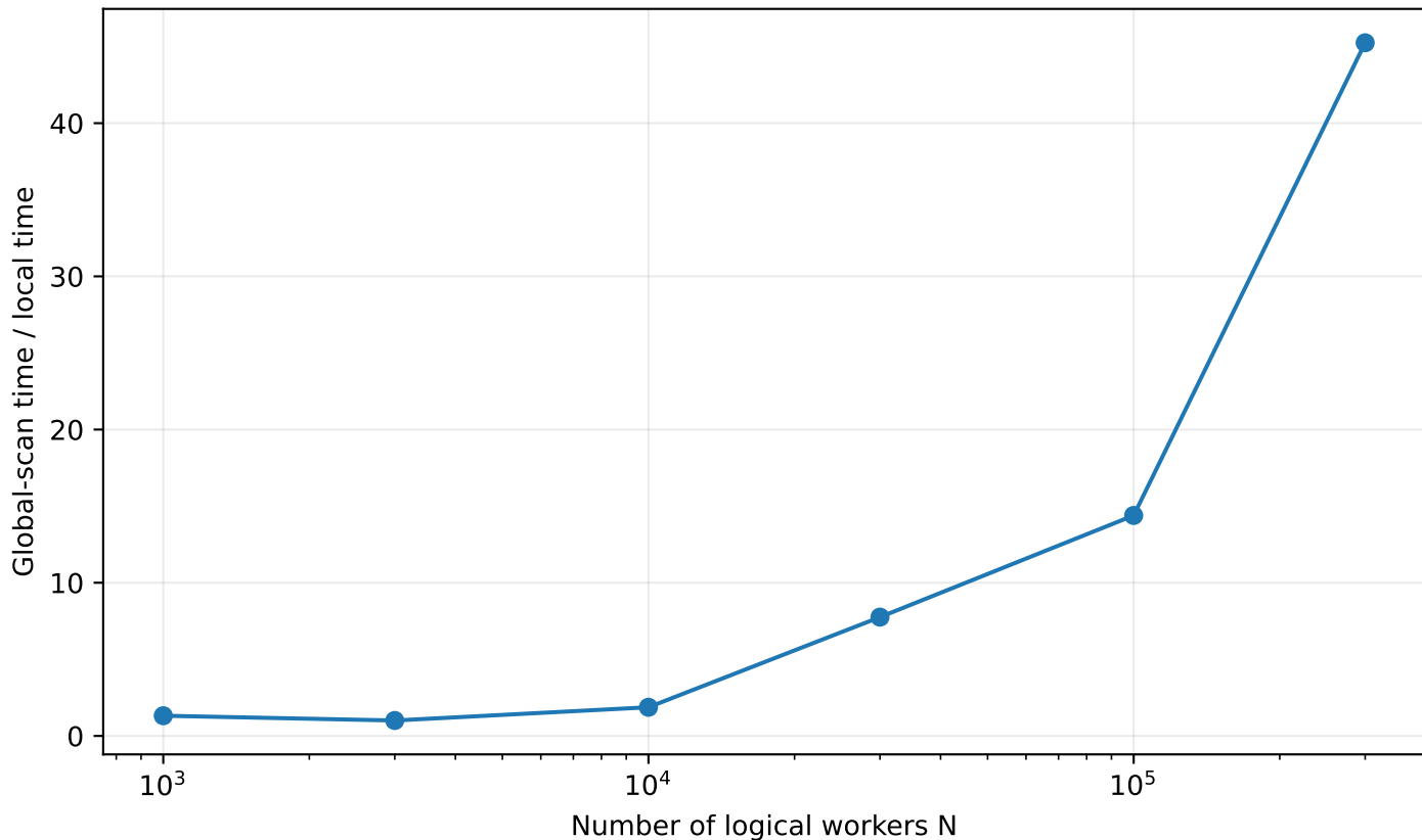
Computational advantage of bounded local candidate generation
