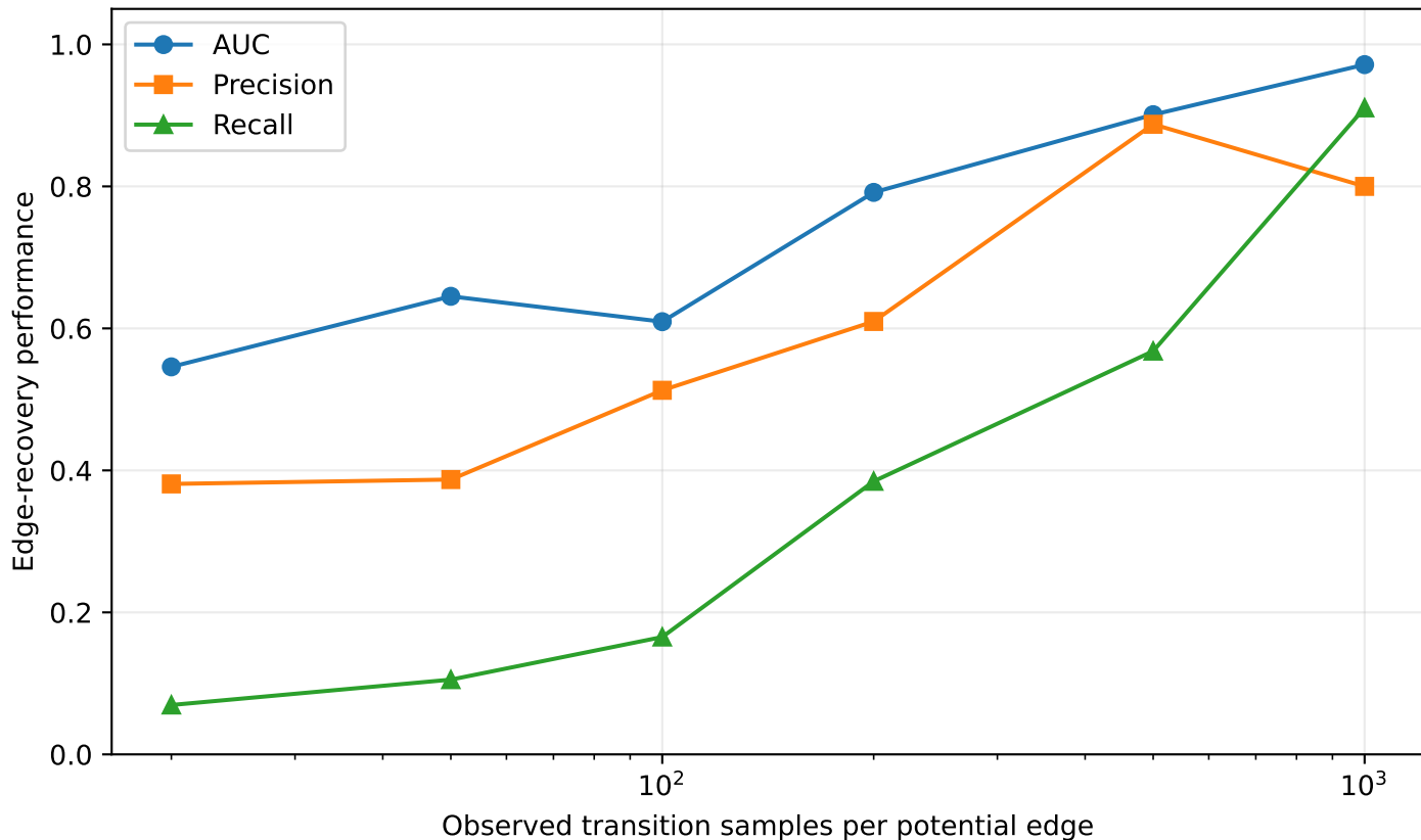
Conditional-information gate recovers informative local edges
