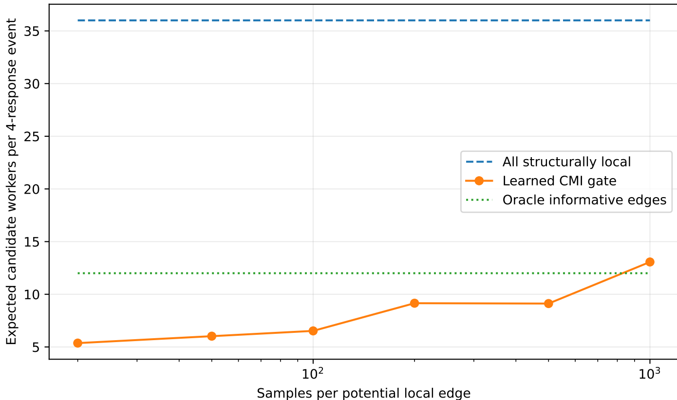
Information gating shrinks the local candidate set
