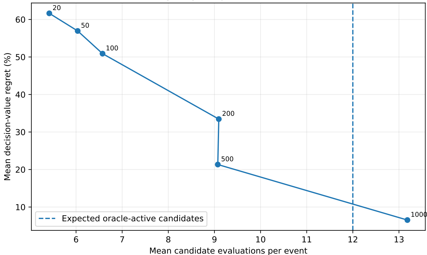
Information-gating compute/decision Pareto curve
