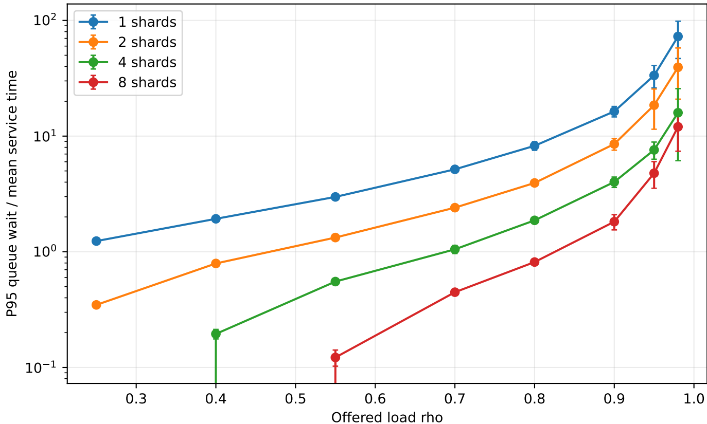
Queue delay with gamma service times
