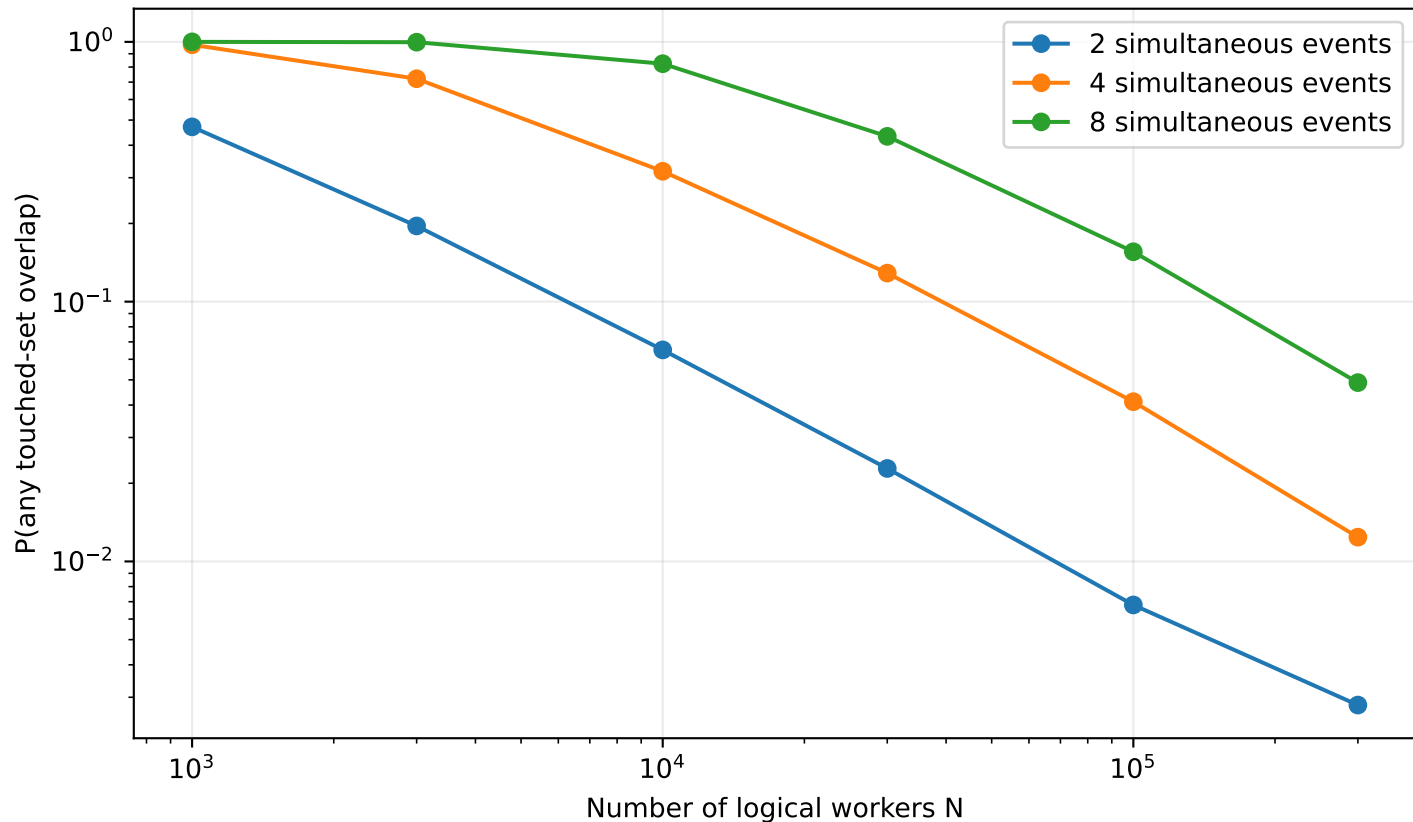
Concurrent local events decouple as the population grows
