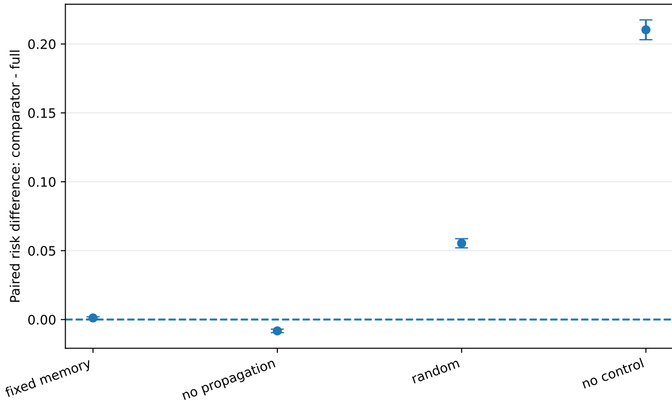
Paired ablation differences with t-based 95% intervals
