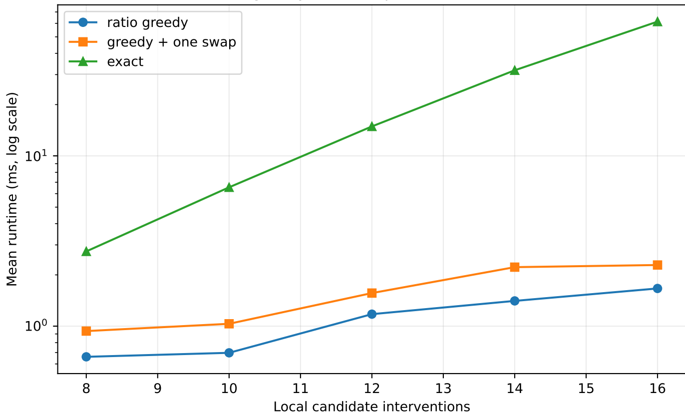
Runtime of greedy, one-swap, and exact local search
