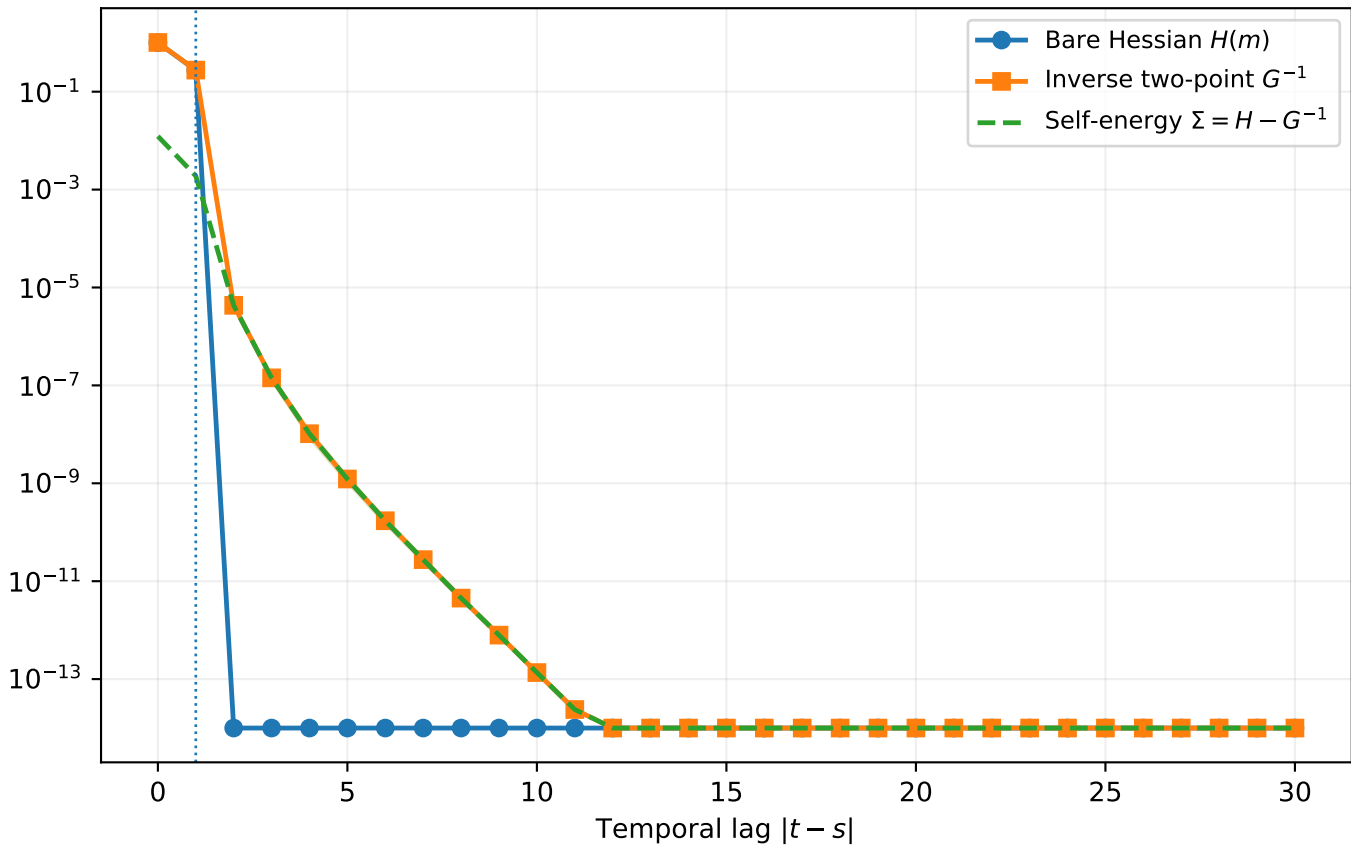
Normalized mean block Frobenius norm
