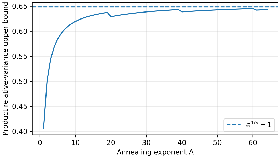
Annealed noise under sufficient B scaling ( c=0.1 )
