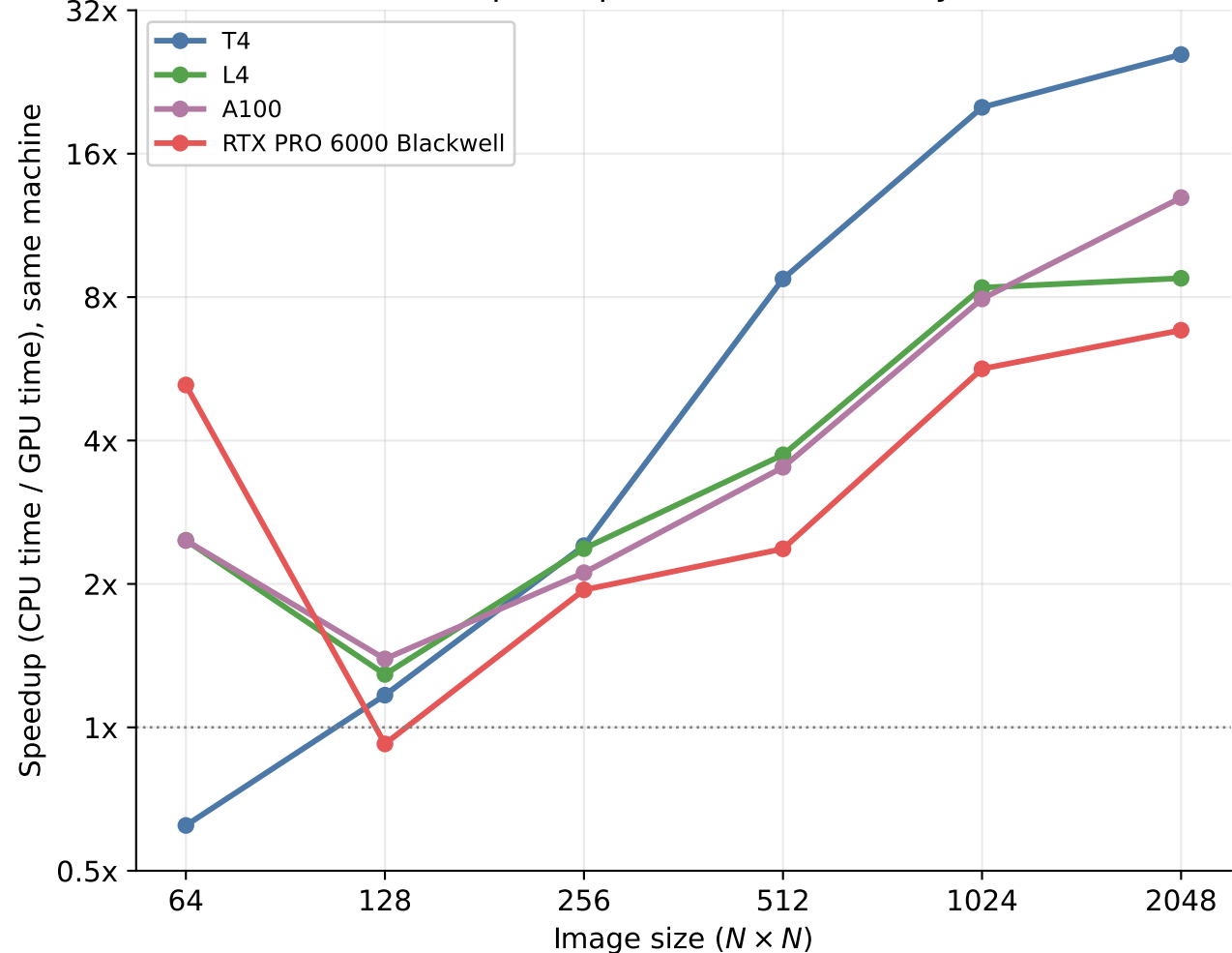
(b) GPU speedup vs. its own CPU, by size
