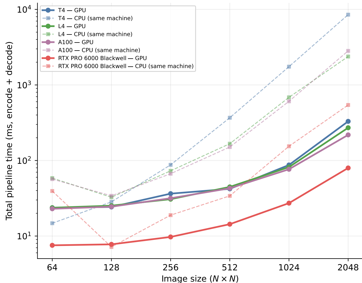
(a) Absolute time vs. size
