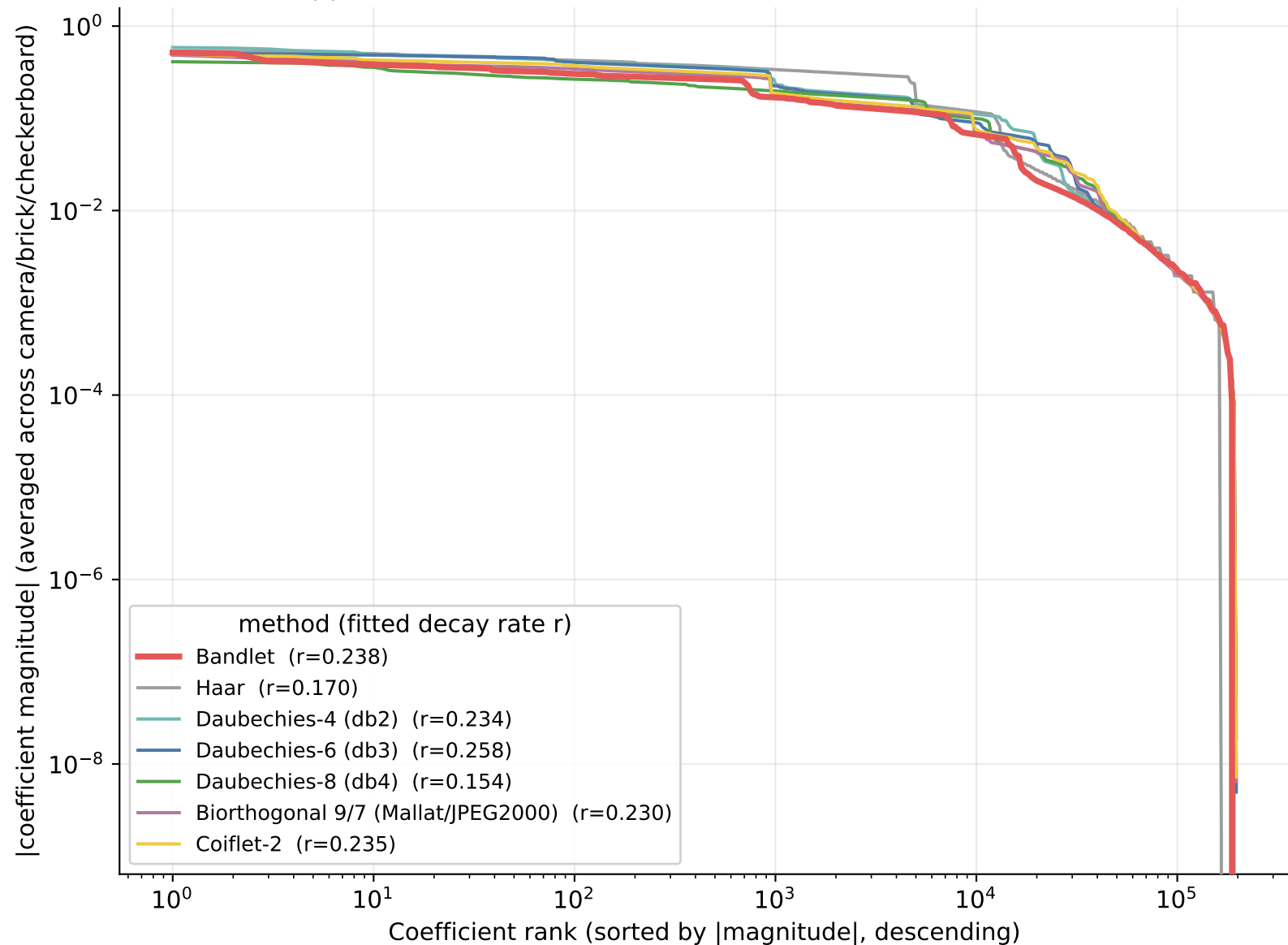
Coefficient-magnitude decay: bandlet vs. classical wavelets |c|_{(n)} \sim n^{-r} fit over rank 10-10,000; steeper decay = sparser
