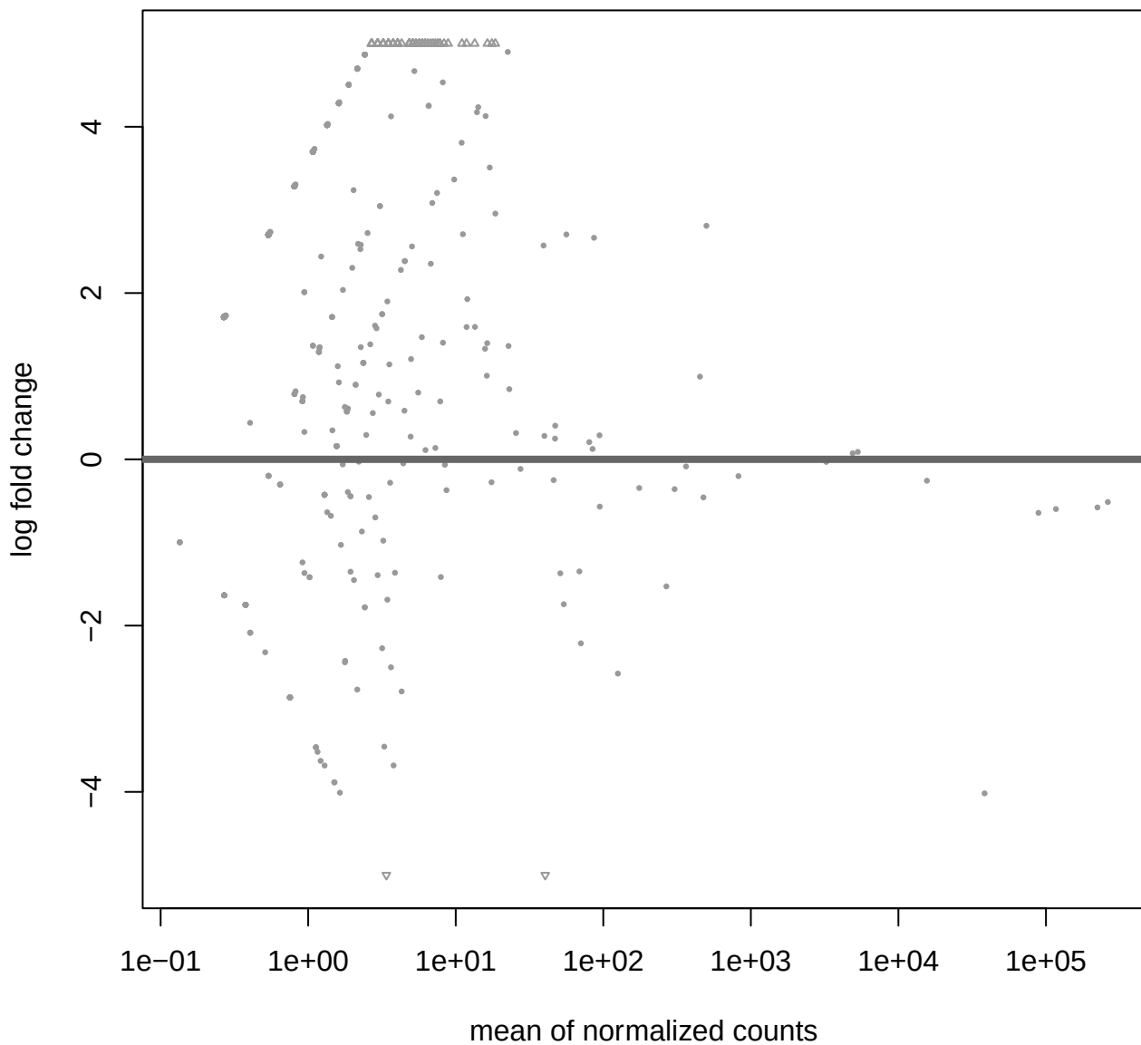
MA Plot (Treatment vs Control)
