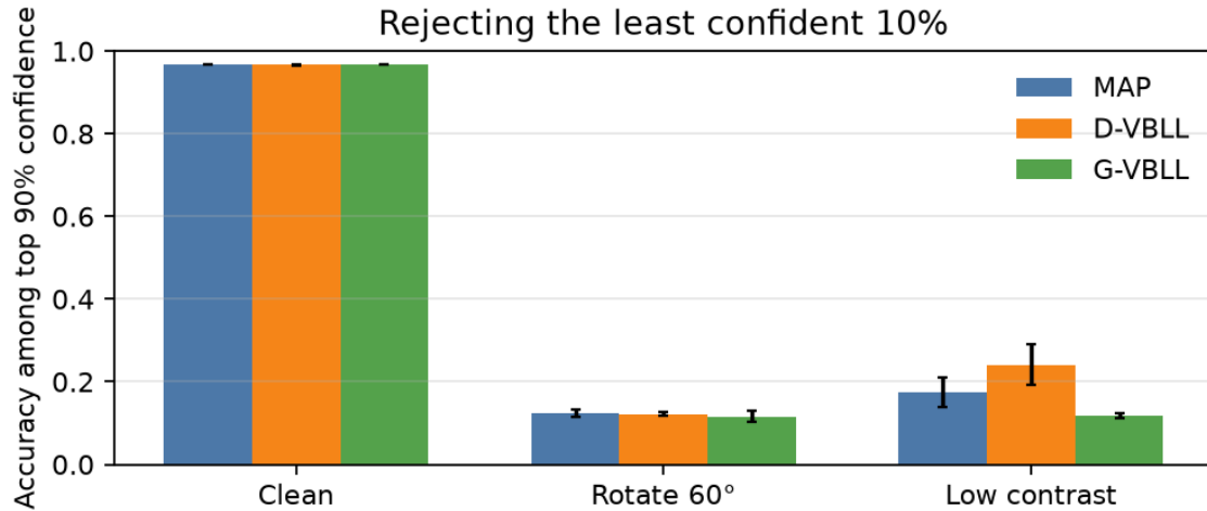
Figure 11: Accuracy after keeping the most confident 90%. The gain exists on clean clothes and disappears under 60^\circ rotation and low contrast.
