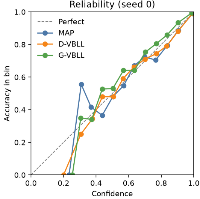
Figure 3: Reliability diagram on the clean test set, seed 0. The three heads sit near the diagonal; D-VBLL is the smoothest of the three.
