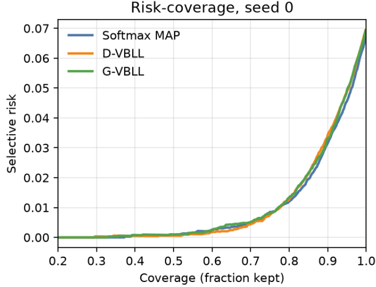
Figure 4: Selective risk against coverage, seed 0. Lower is better. The three curves overlap: all heads become accurate once low-confidence predictions are refused.
