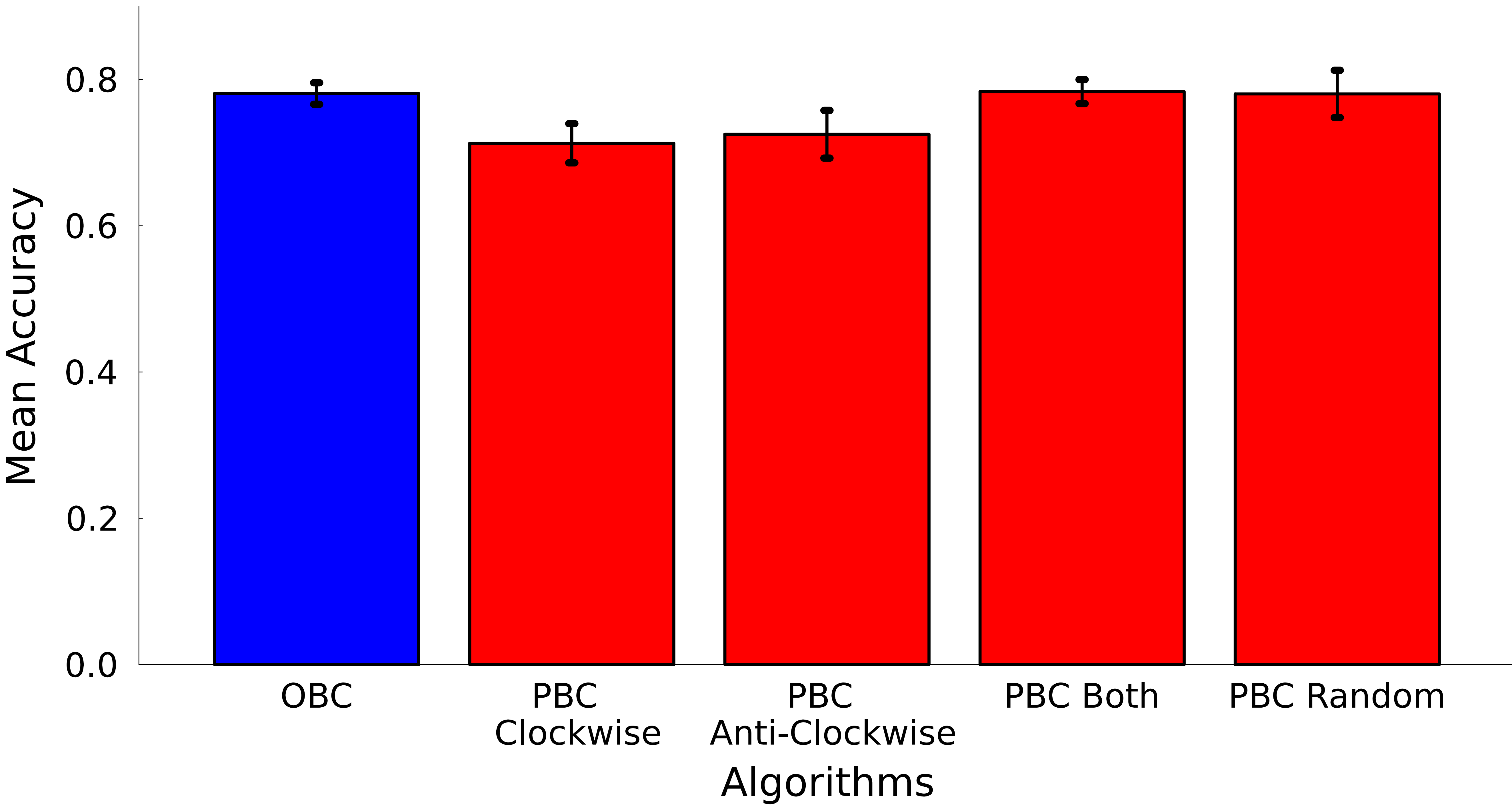
Comparison of Algorithms for ArrowHead Dataset: \chi_{max} = 16 , \eta = 0.2 , d = 4 , Legendre Encoding, Averaged Across 20 Seeds
