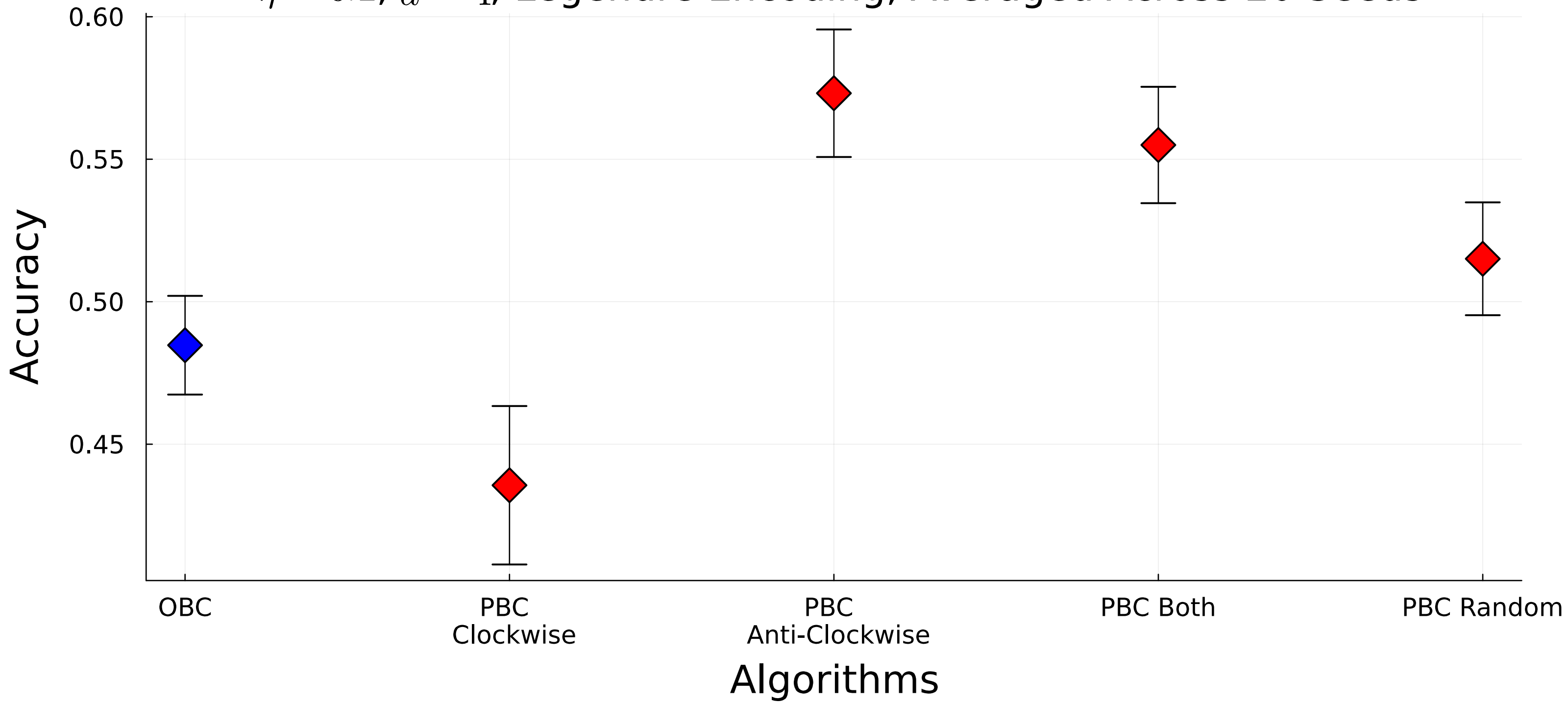
Comparison of Algorithms for Medical Image Dataset: \chi_{max} = 16 , \eta = 0.2 , d = 4 , Legendre Encoding, Averaged Across 20 Seeds
