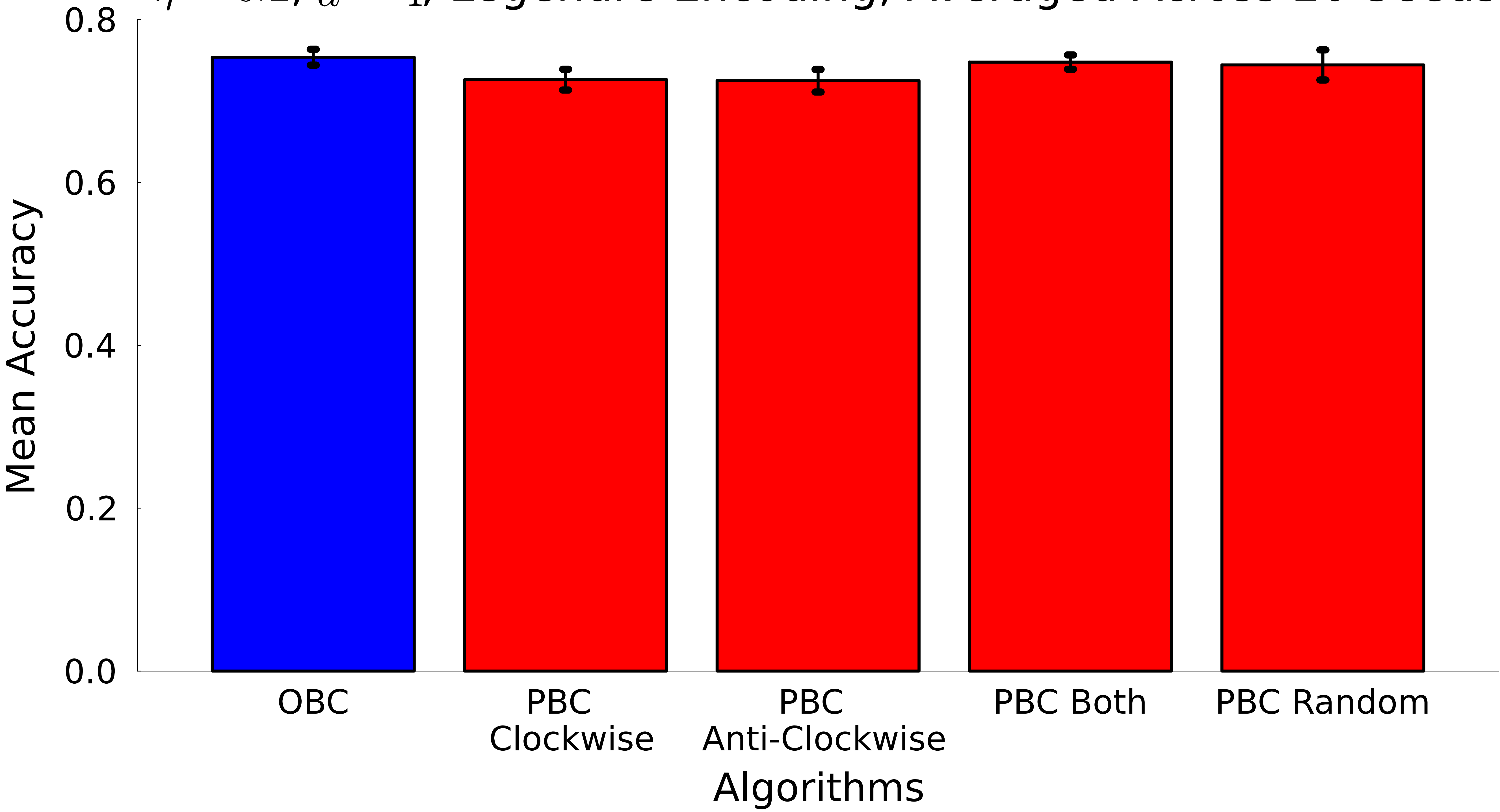
Comparison of Algorithms for Swedish Leaf Dataset: \chi_{max} = 16 , \eta = 0.2 , d = 4 , Legendre Encoding, Averaged Across 20 Seeds
