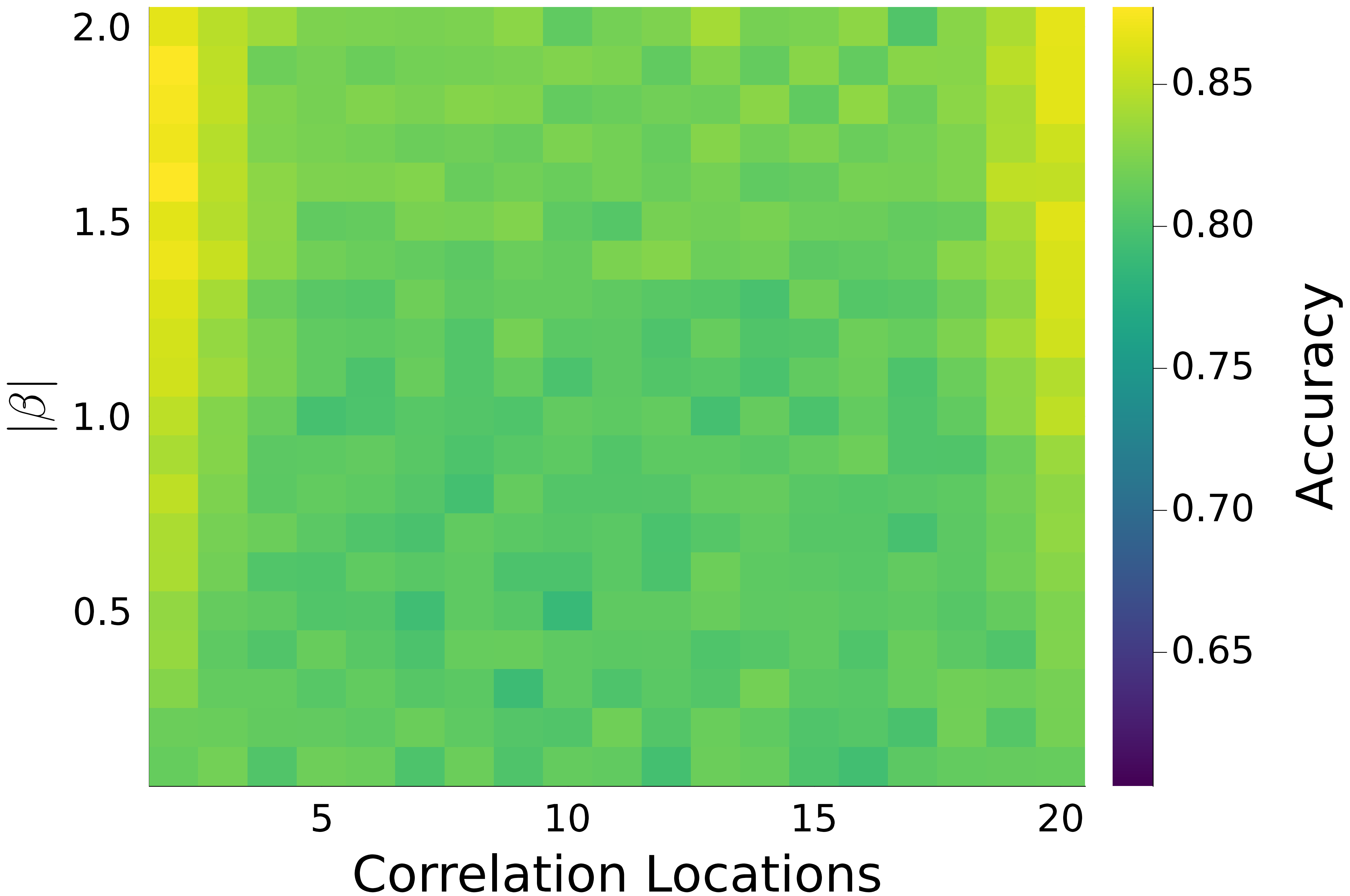
Test Accuracy Heatmap, PBC \alpha_A, \alpha_B = \pm 0.4, \beta_A = -\beta_B, \chi_{max} = 3 Averaged Across 40 Seeds
