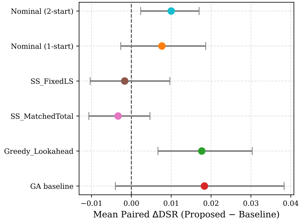
(b) Cross-Scenario Paired \Delta DSR (95% Scenario Bootstrap CI)
