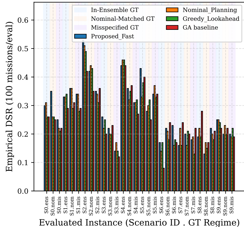
(a) Performance Across 30 Evaluations (10 Scenarios \times 3 GT Regimes)
