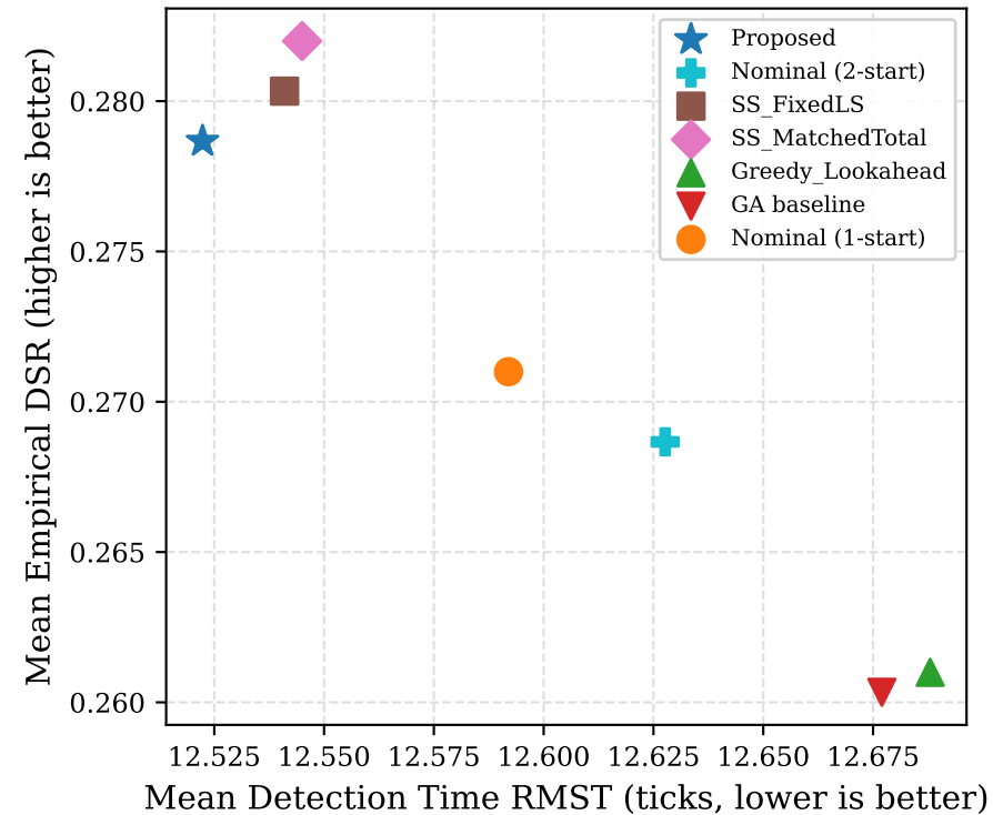
(c) Multi-Objective Quality (DSR vs. RMST)
