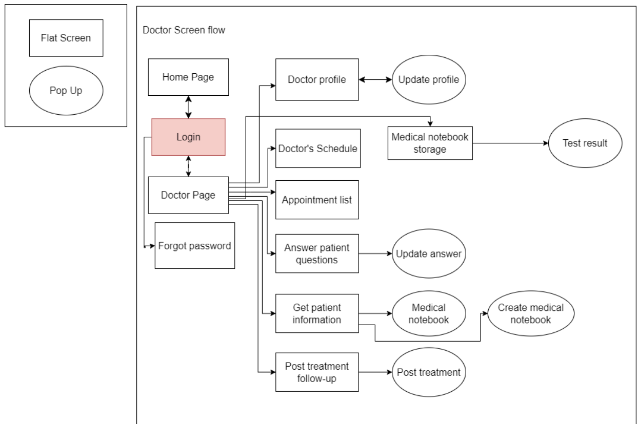
Figure 1.4.2.1 Doctor screen flow
