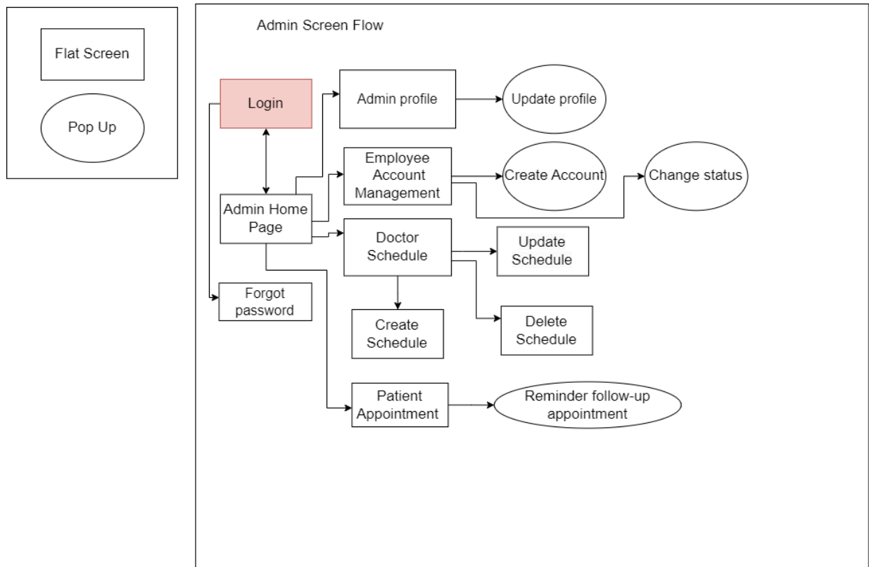
Figure 1.4.5.1 Admin screen flow
