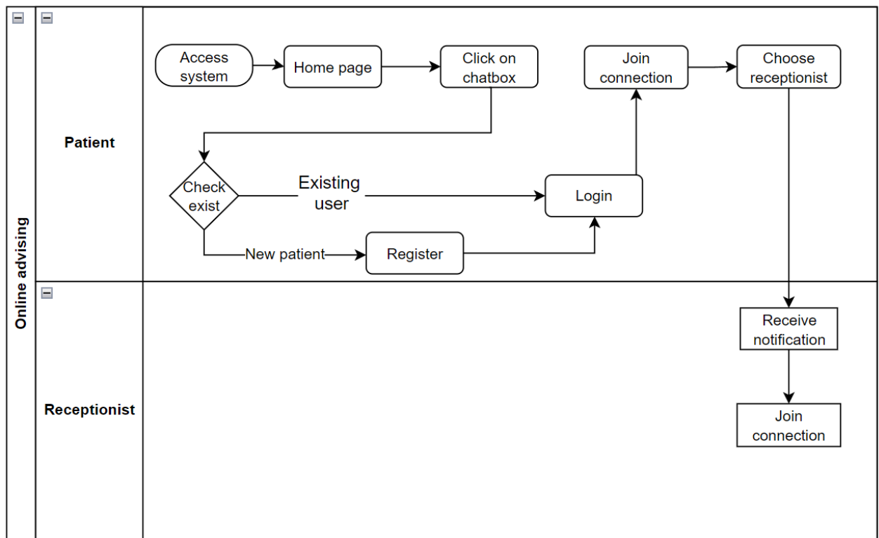
Figure 1.2.2.2 Online advising workflow
