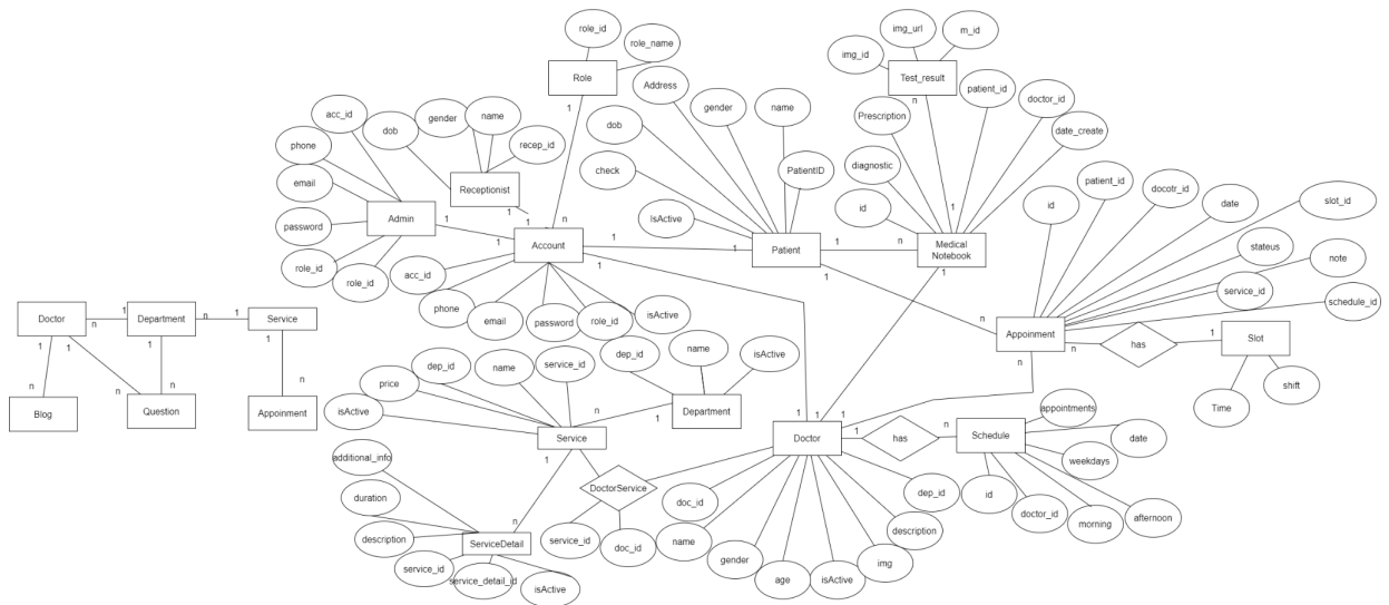
Figure 1.5.1 Entity Relationship Diagram
