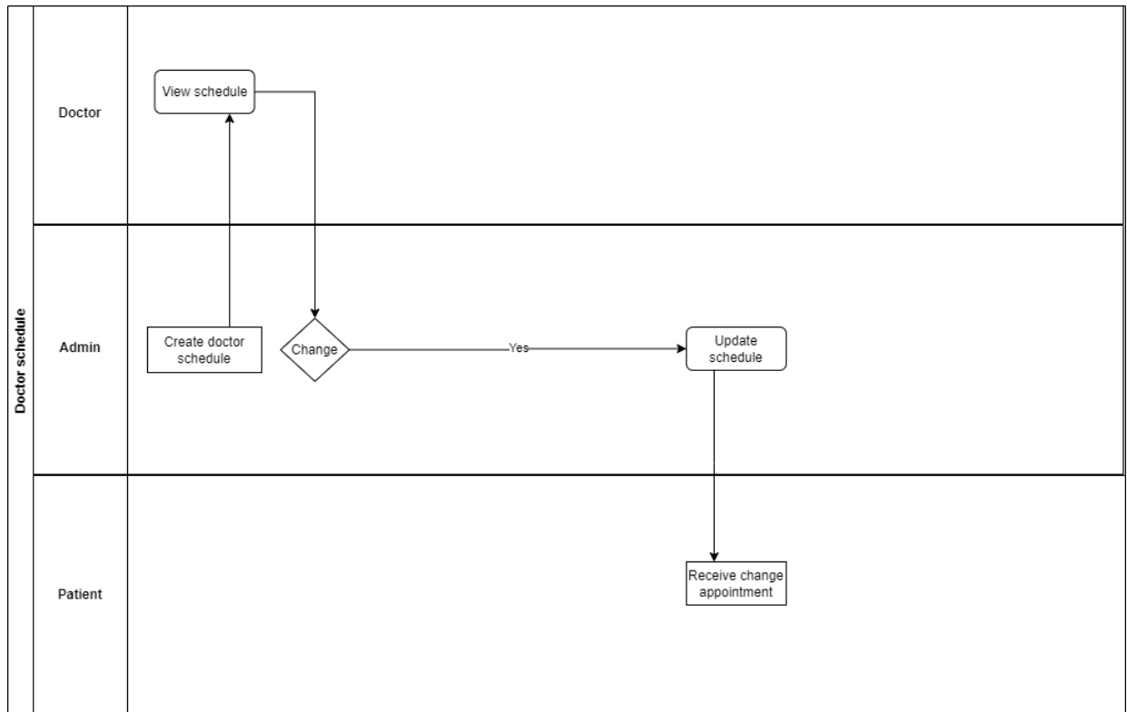
Figure 1.2.4.1 Doctor schedule workflow
