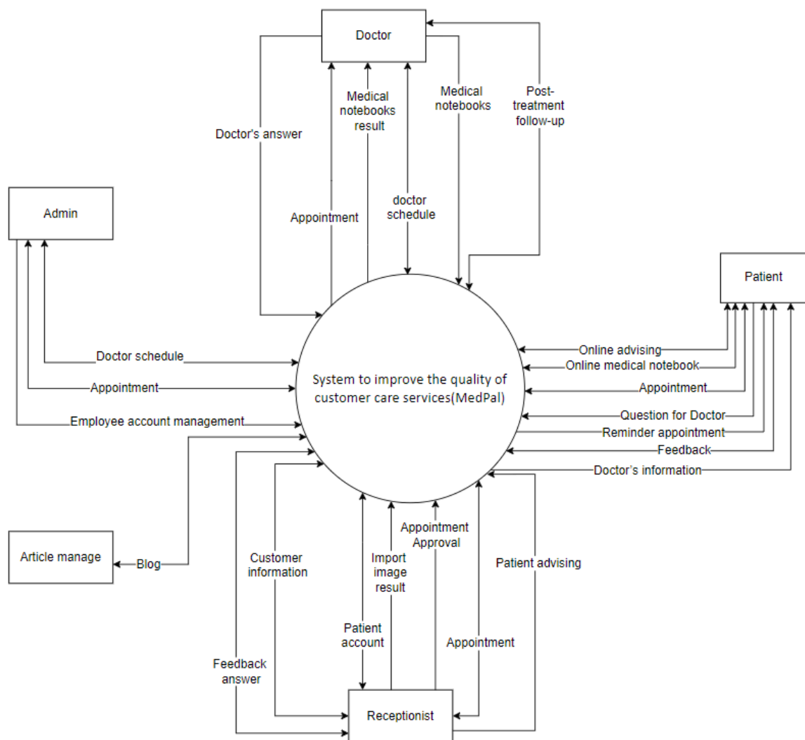
Figure 1.1.1 MedPal Context diagram
