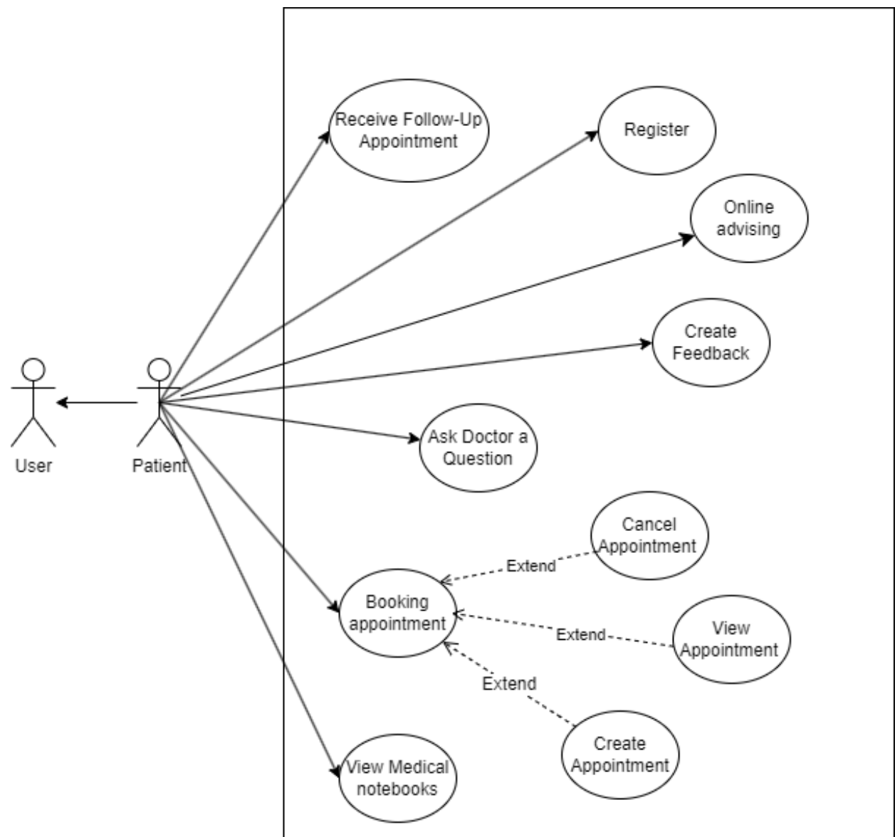
Figure 1.3.2.3.1 Patient use case diagram
