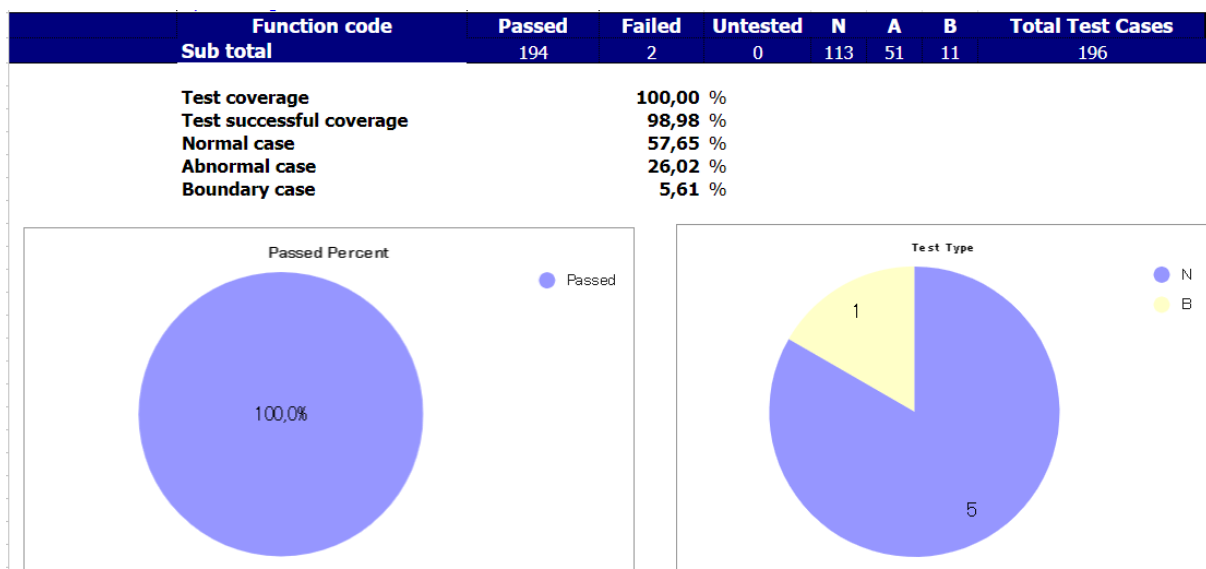
Figure 5.1.1 Unit test
