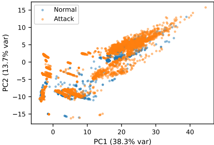
PCA Projection of RT-IoT Traffic
