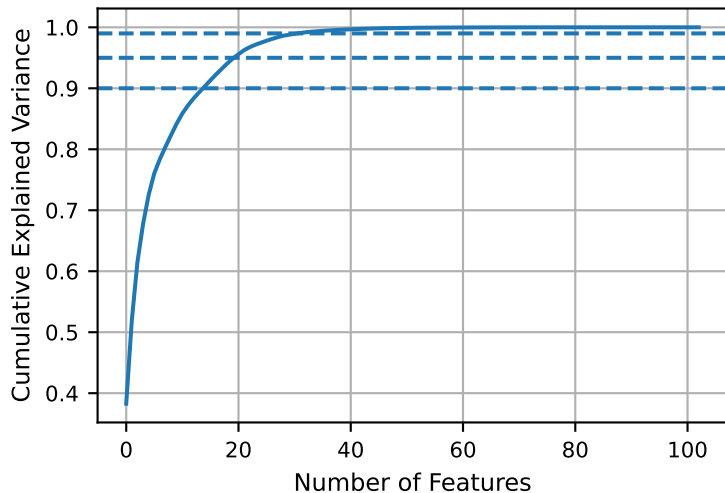
Cumulative Explained Variance (standardized numeric features)
