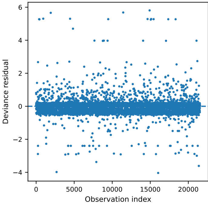
Deviance Residual Diagnostic
