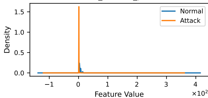
fwd_subflow_pkts
