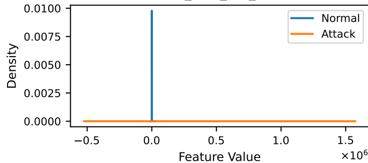
bwd_pkts_per_sec
