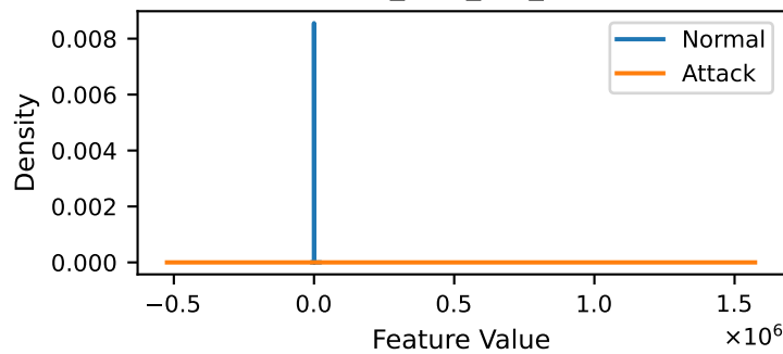
payload_bytes_per_second
