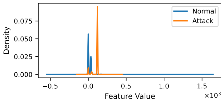
fwd_init_window_size
