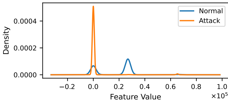
active.min
