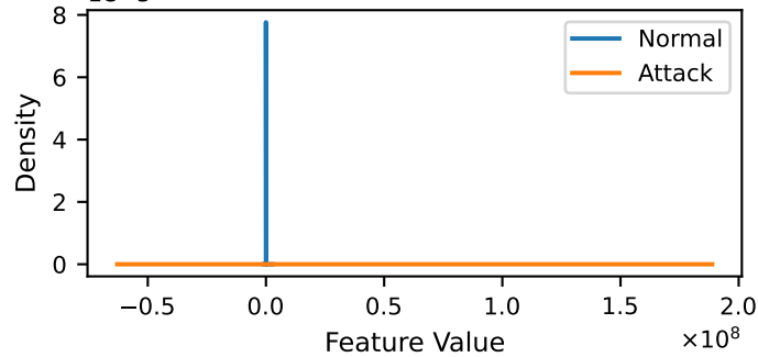
fwd_subflow_pkts
