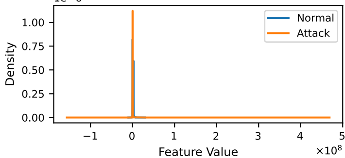
active.min
