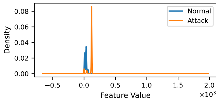
fwd_pkts_per_sec
