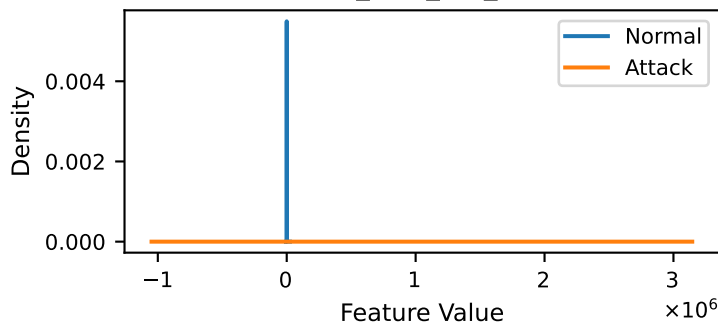
bwd_init_window_size
