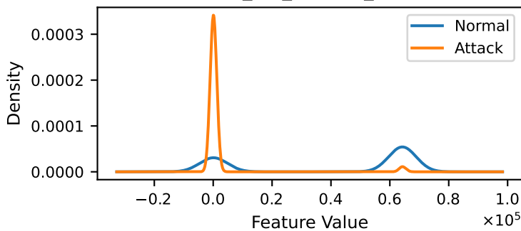
flow_pkts_per_sec
