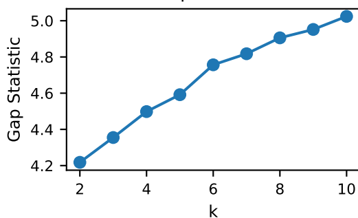
Gap Statistic
