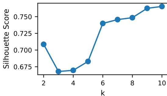
Silhouette Score
