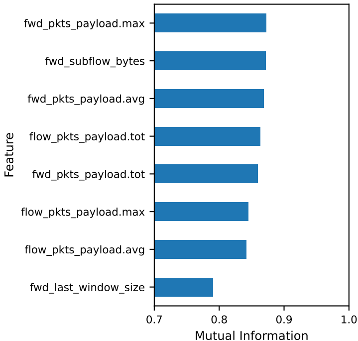
Top Predictive Features (Mutual Information) ( > 0.7 )
