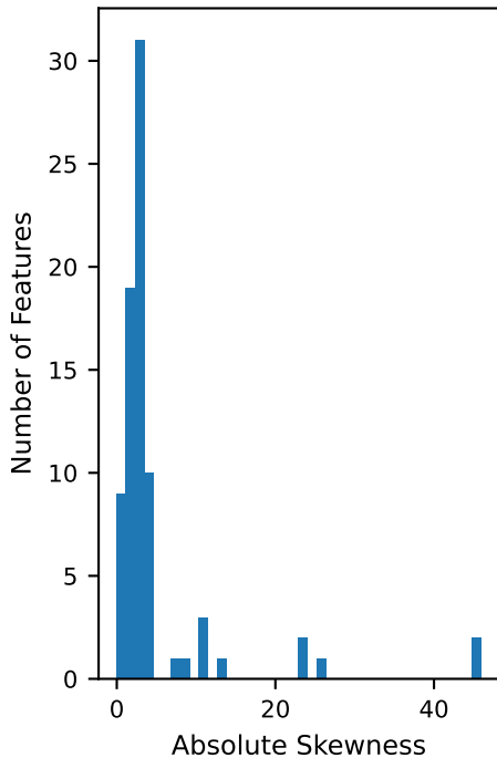
Log-Transformed Feature Skewness
