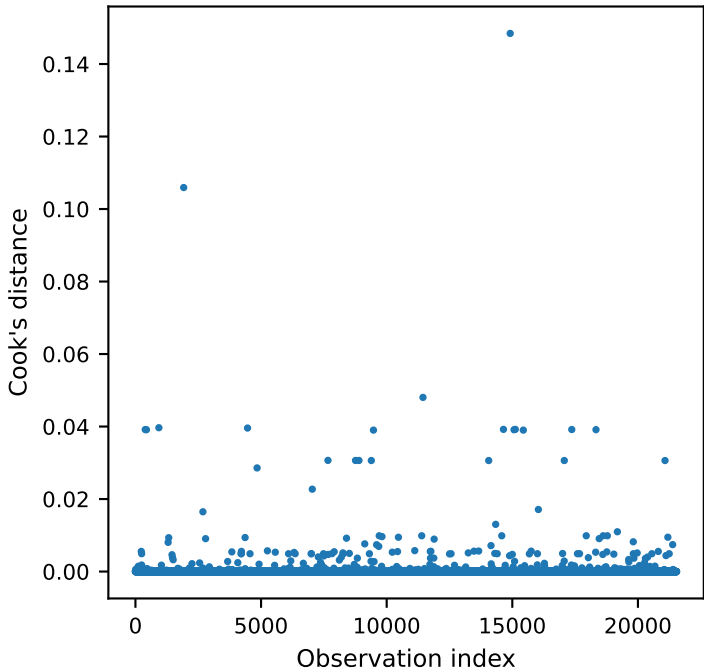
Influential Observation Diagnostic
