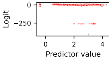
bwd_iat.avg
