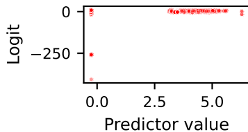
bwd_pkts_payload.min
