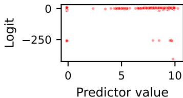
fwd_header_size_min
