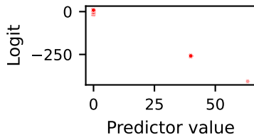
flow_ECE_flag_count
