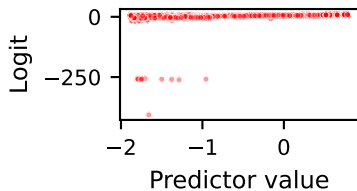
flow_pkts_per_sec
