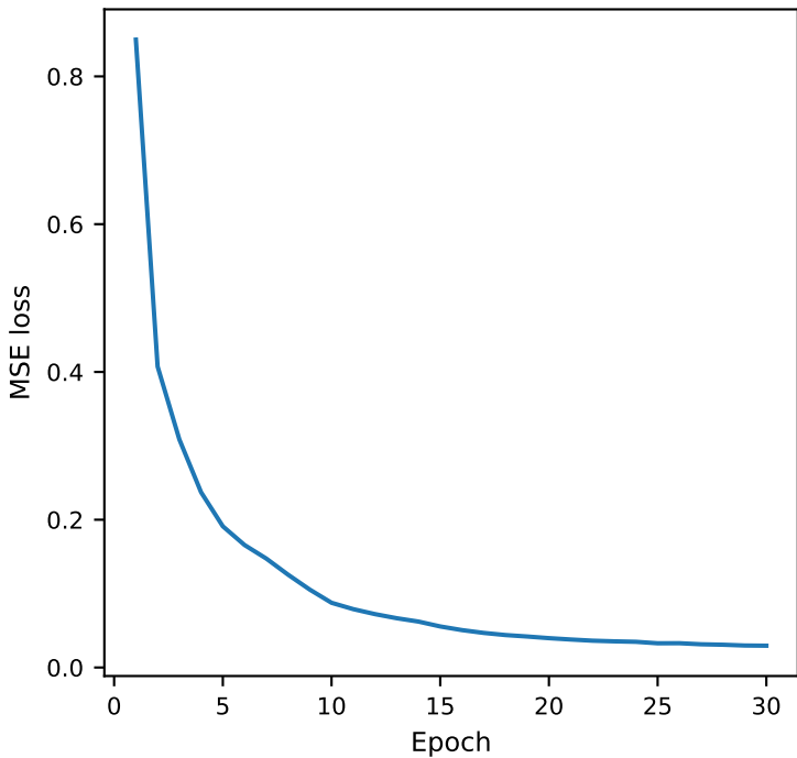
Baseline AE Training Loss
