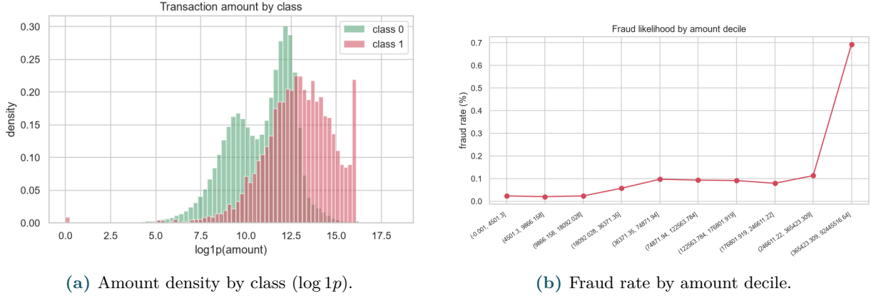
Figure 3.3: Transaction amount vs. fraud likelihood. Fraud concentrates in large amounts.
