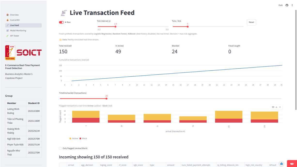
Figure A.2: Live Feed: a simulated real-time stream scored by all three models with the max-risk aggregate decision; running counters (received / in review / blocked / fraud caught) and the review-versus-block timeline.
