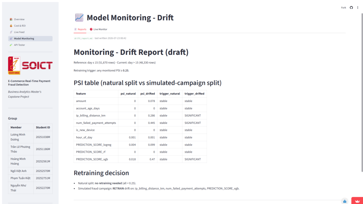
Figure A.4: Monitoring page (Reports tab): the committed drift report. The PSI table contrasts a natural day-split (all stable ) with a simulated fraud campaign, which trips the retraining trigger (PSI ≥ 0.25) on ip_billing_distance_km , num_failed_payment_attempts , and PREDICTION_SCORE_xgb .
