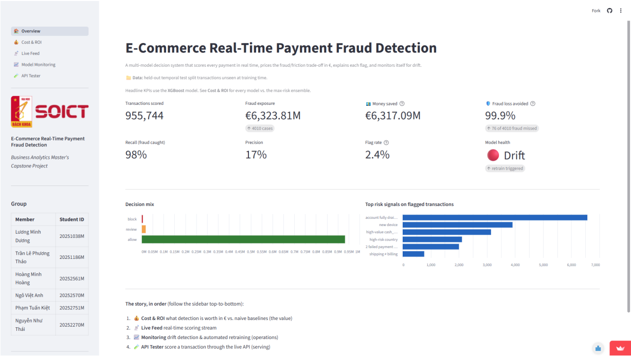
Figure A.1: Overview page: headline KPIs (money saved, fraud loss avoided 99.9%, recall 98%, precision 17%, flag rate 2.4%, and a “drift” model-health flag), the allow/review/block decision mix, and the top risk signals on flagged transactions. All metrics are on the held-out test split.
