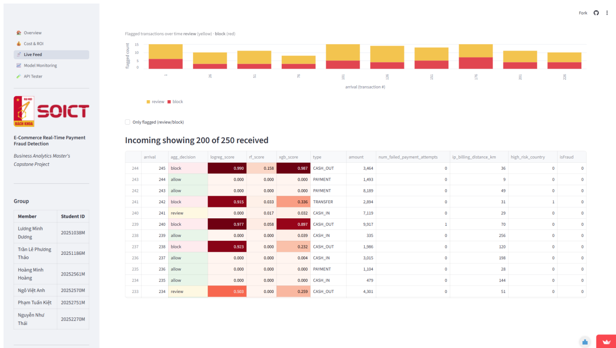
Figure A.3: Live Feed transaction table: per-model scores ( logreg_score , rf_score , xgb_score ), the aggregated allow/review/block decision, and the raw features. Rows where one model is confident while another is not are still escalated by the max-risk rule.
