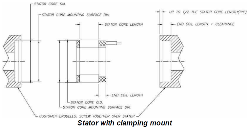
Figure 4: Axial Clamping of Stator [2]
