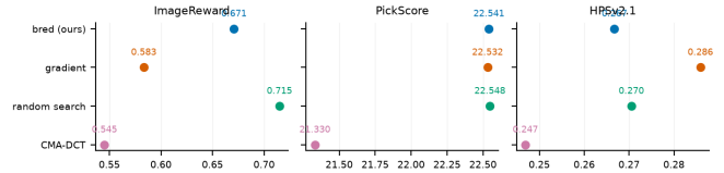
Figure 2: Preference-model judges (higher is better), averaged over prompts. None of these models appears in any method’s objective.
