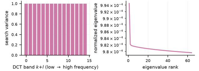
Figure 3: Left: CMA-adapted search variance by DCT band k+l , averaged over prompts. Right: covariance eigenvalue decay.
