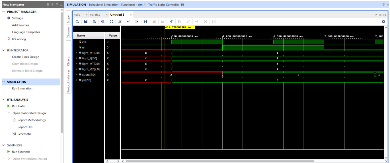
Figure 6.3 : Output Waveform
