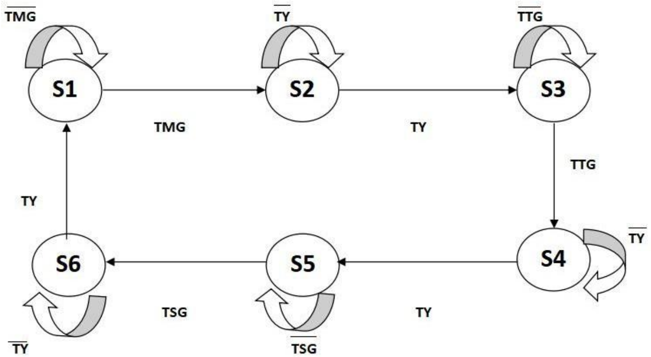
Figure 3.3 : State Diagram
