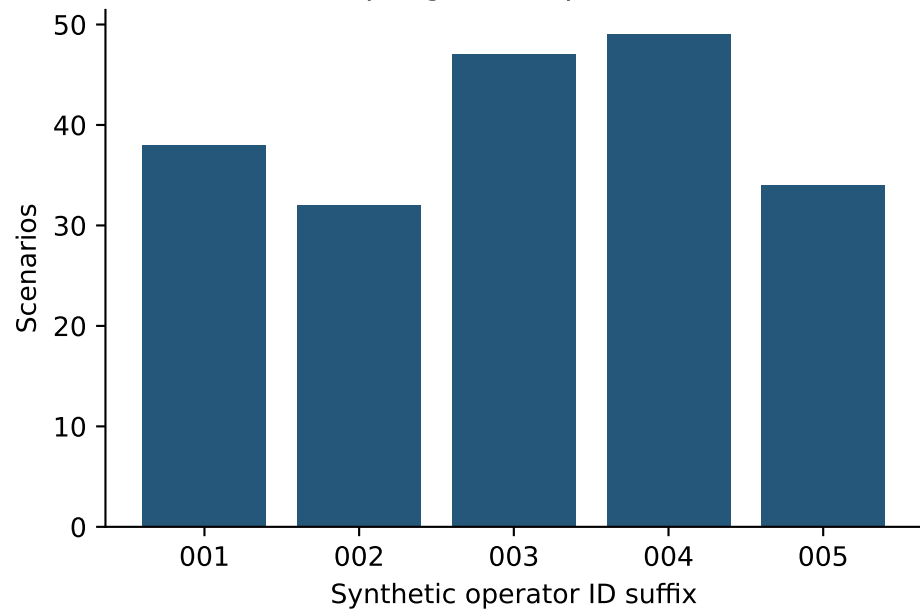
Sampling with replacement
