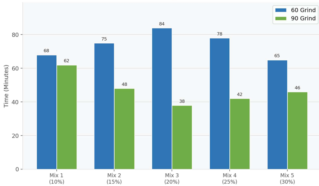
Initial Setting Time (IST)
