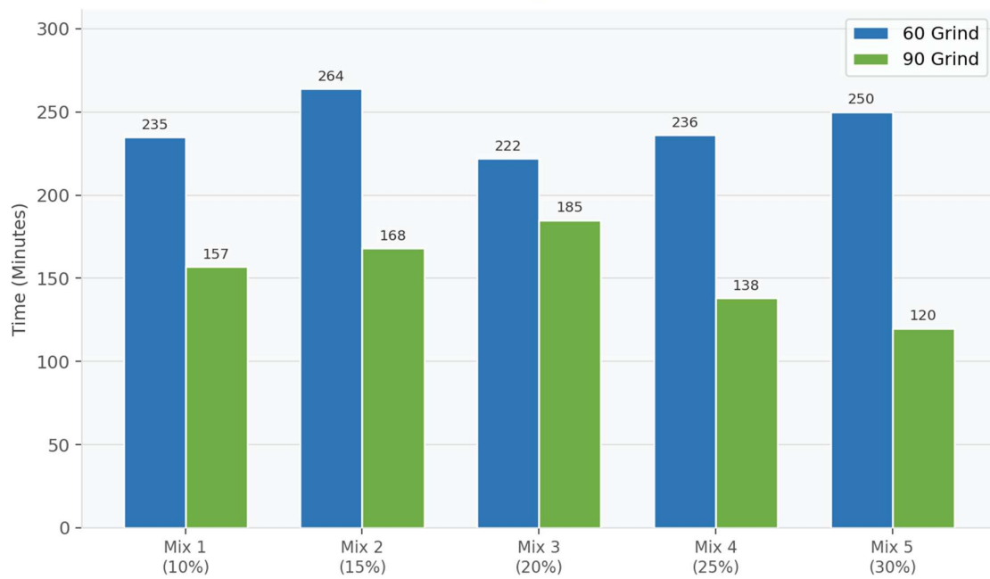
Final Setting Time (FST)
