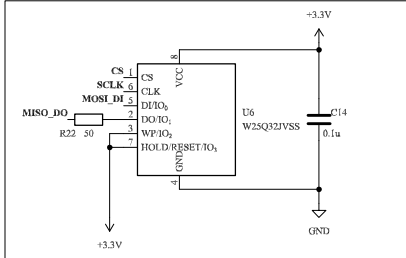
Flash Memory
