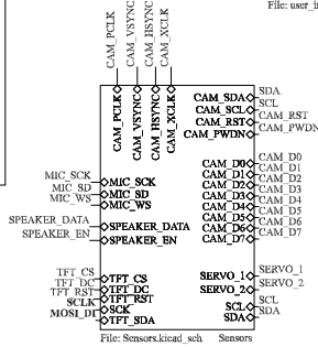
File: Sensors.kicad_sch Sensors
