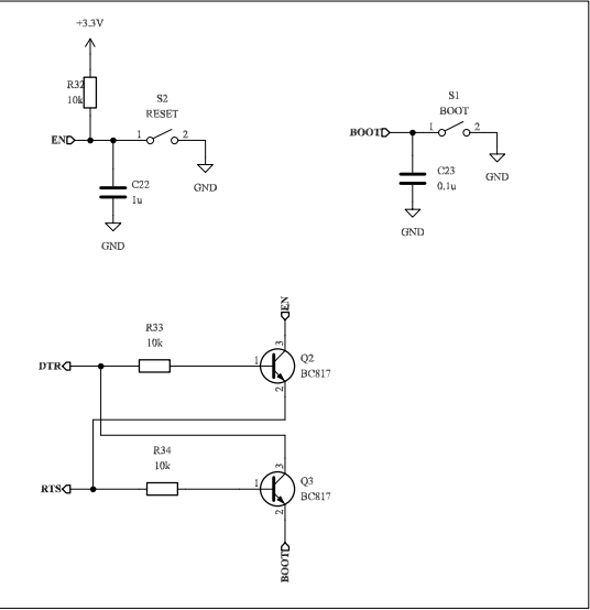
BOOT and RESET Button
