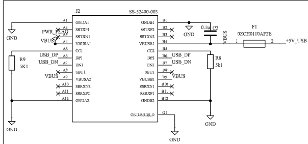
USB-C Connector
