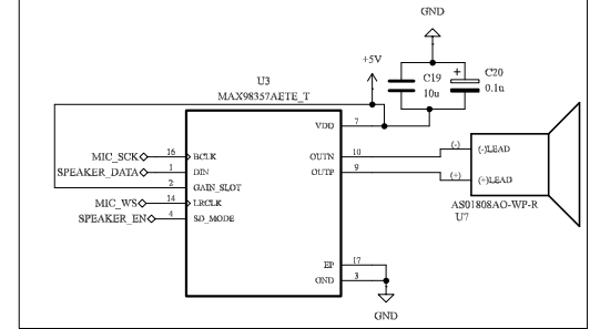
Speaker and Amplifier
