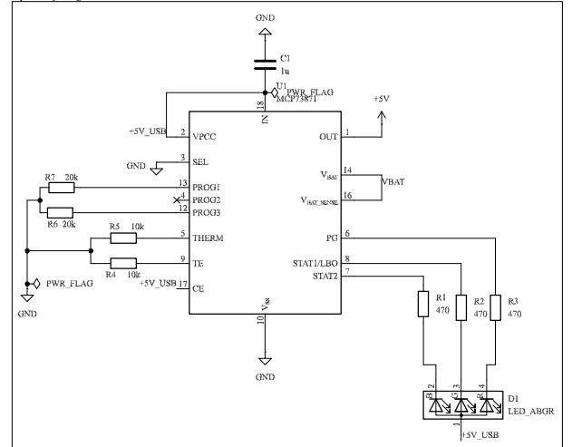
Lipo Battery Charger
