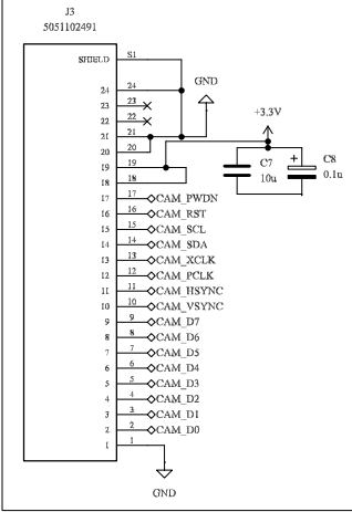
Camera Connector
