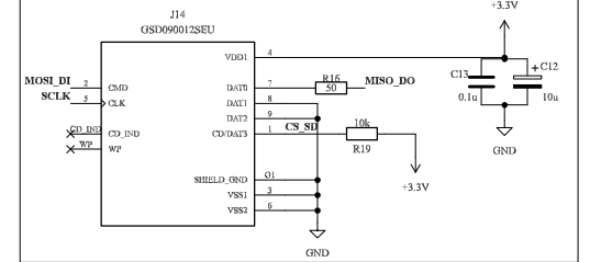
SD Card Module
