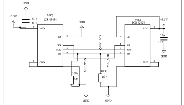
Microphone
