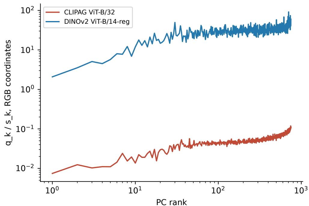
CLIPAG ViT-B/32 vs DINOv2 ViT-B/14-reg | 10 fixed seeds different architectures / selected layers; separate training PCA750; RGB metric
